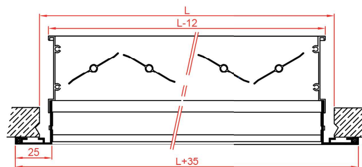
SDG with opposite blade damper (OBD)
