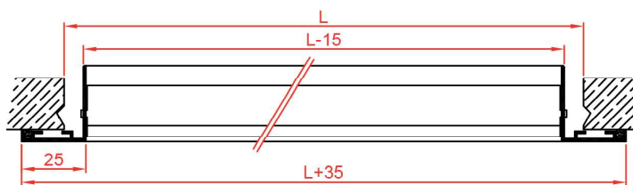
SDG with opposite blade damper (OBD)
